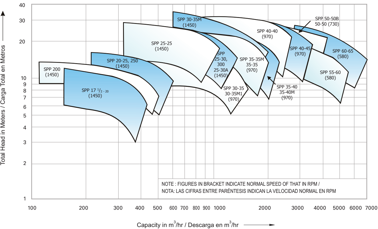
Family Curve of MF Pump at 50 Hz rpm / Familia de curvas de Bomba SPP - 50 Hz
